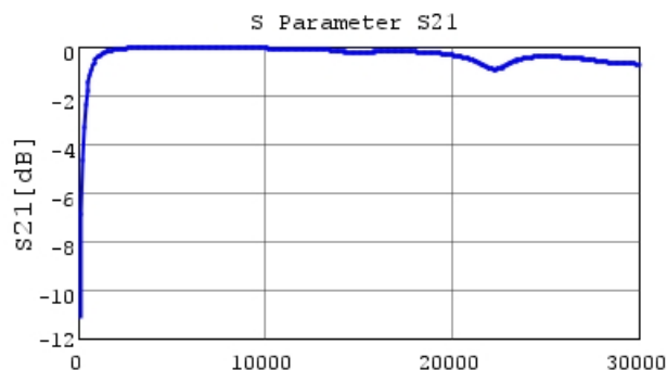
GRM0225C1H4R6CA03 S21 DCOV, 25degC
