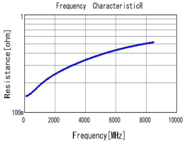
■ GRM0225C1H6R1BA03 R DCOV, 25degC
