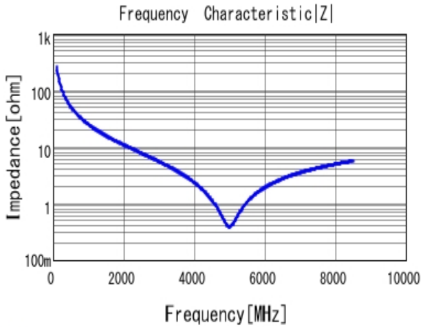
■ GRM0225C1H6R1BA03 |Z| DCOV, 25degC
