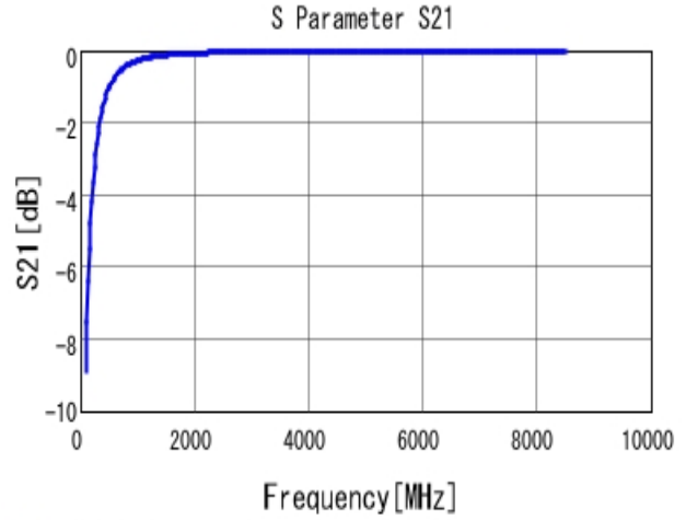
■ GRM0225C1H6R1BA03 S21 DCOV, 25degC
