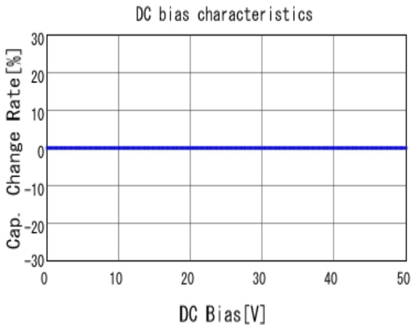
■ GRM0225C1H6R1BA03 C-DC bias capchange, 25.0degC, AC1V
