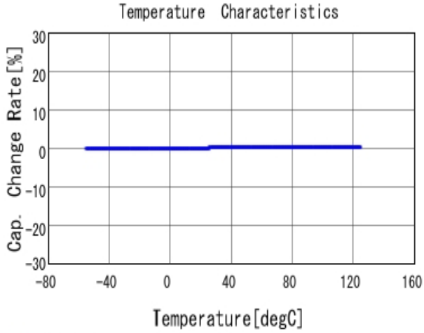
■ GRM0225C1H6R1BA03 C-Temp. capchange, DCOV, AC1Vrms
