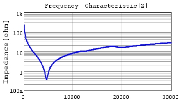
GRM0225C1H7R2WA03 |Z| DCOV,25degC
