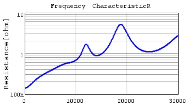
GRM0225C1H7R2WA03 R DCOV,25degC
