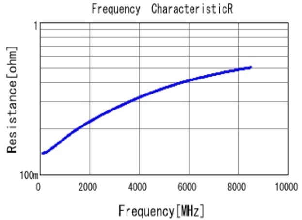
■ GRM0225C1H7R9CA03 R DC0V, 25degC
