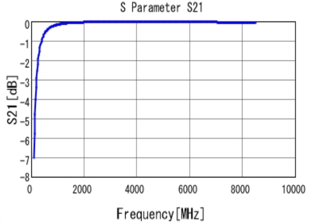
■ GRM0225C1H7R9CA03 S21 DCOV, 25degC
