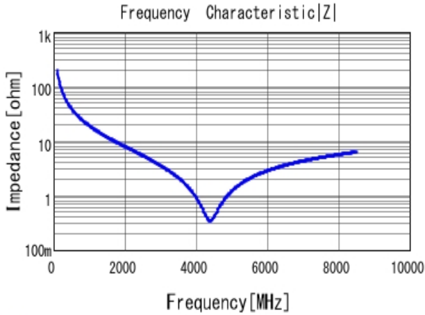
■ GRM0225C1H7R9CA03 |Z| DC0V, 25degC
