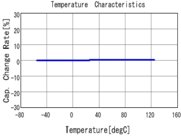
■ GRM0225C1H7R9CA03 C-Temp. capchange, DCOV, AC1Vrms
