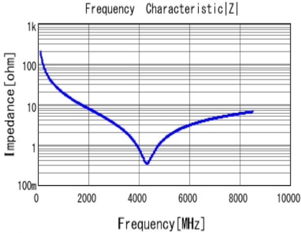
■ GRM0225C1H8R0DA03 |Z| DCOV, 25degC
