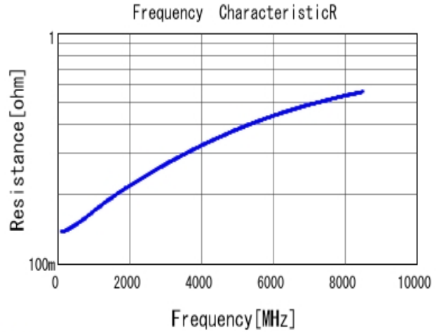
■ GRM0225C1H8R0DA03 R DCOV, 25degC
