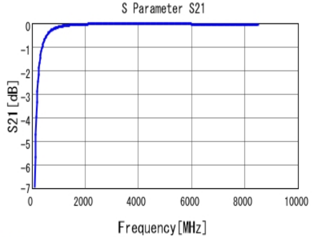
■ GRM0225C1H8R0DA03 S21 DCOV, 25degC
