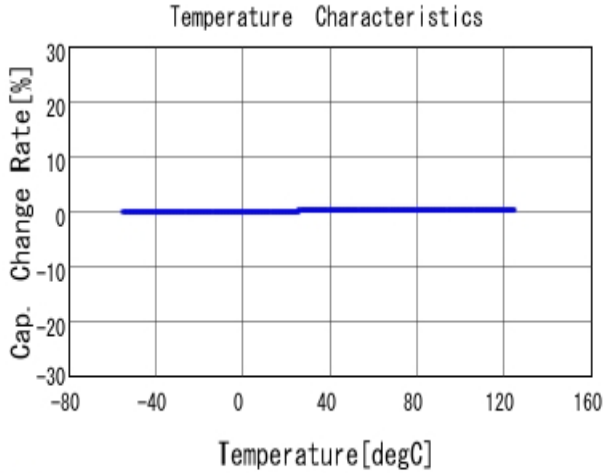
■ GRM0225C1H8R0DA03 C-Temp. capchange, DCOV, AC1Vrms
