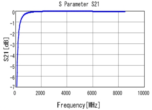
■ GRM0225C1H8R0WA03 S21 DCOV, 25degC
