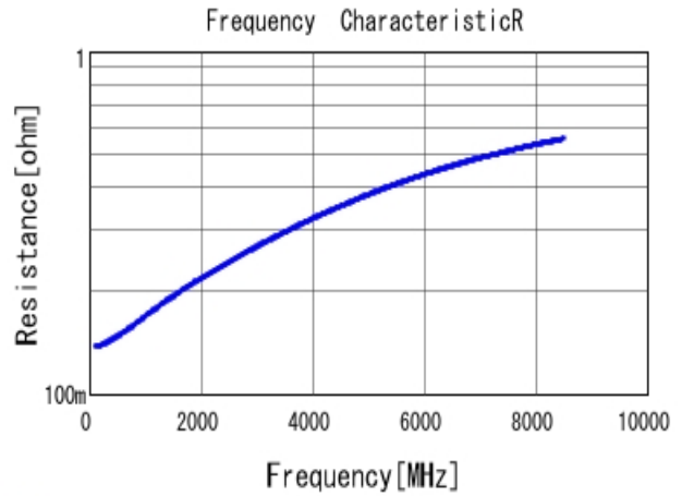
■ GRM0225C1H8R0WA03 R DCOV, 25degC
