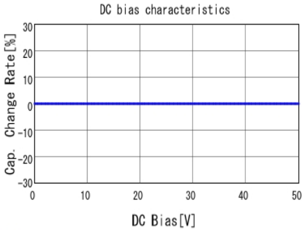
■ GRM0225C1H8R0WA03 C-DC bias capchange, 25.0degC, AC1V
