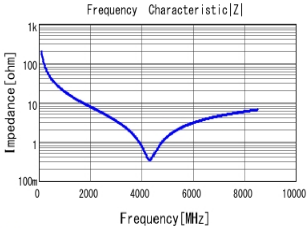
■ GRM0225C1H8R0WA03 |Z| DCOV, 25degC
