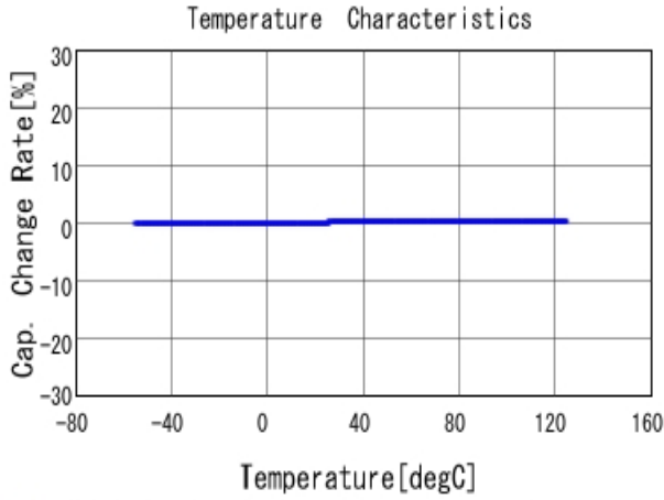
■ GRM0225C1H8R0WA03 C-Temp. capchange, DCOV, AC1Vrms
