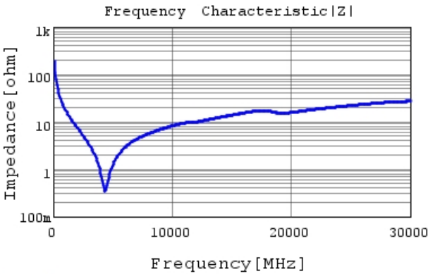
GRM0225C1H8R3WA03 |Z| DCOV,25degC
