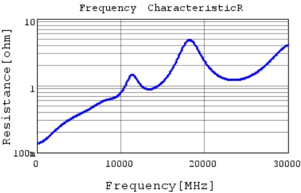
GRM0225C1H8R3WA03 R DCOV,25degC
