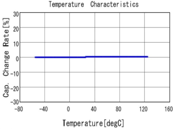
■ GRM0225C1H9R5BA03 C-Temp. capchange, DCOV, AC1Vrms
