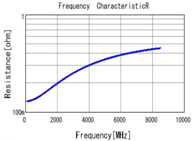
■ GRM0225C1H9R5BA03 R DCOV, 25degC
