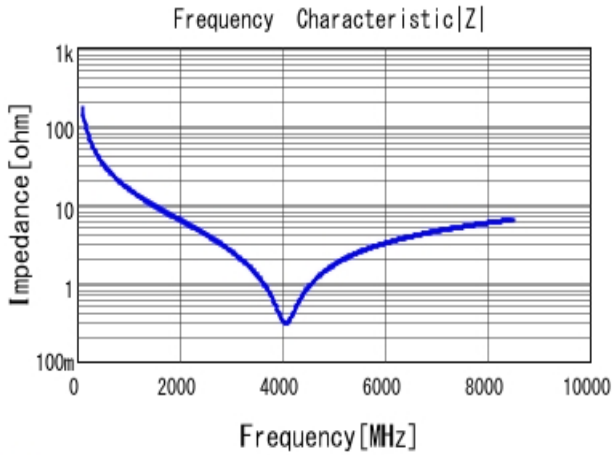
■ GRM0225C1H9R5BA03 |Z| DCOV, 25degC
