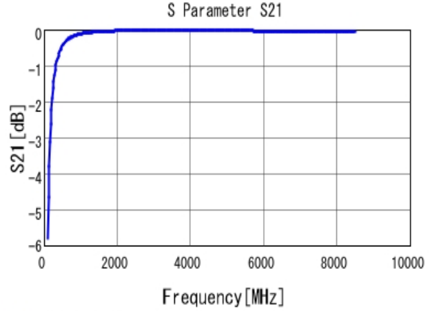
■ GRM0225C1H9R5BA03 S21 DCOV, 25degC
