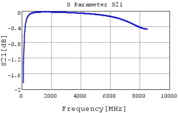
GRM0332C2A220GA01 S21 DCOV, 20degC
