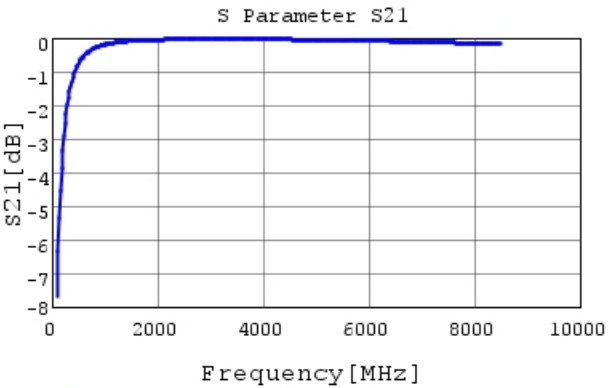
GRM0332C2A7R2BA01 S21 DCOV, 20degC
