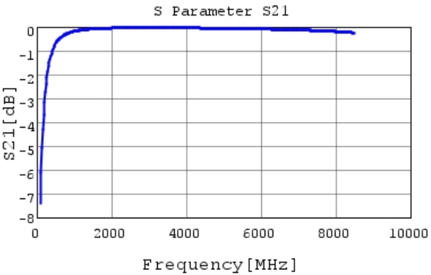
GRM0332C2A7R5CA01 S21 DCOV, 20degC
