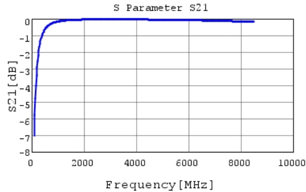
GRM0332C2A7R9WA01 S21 DCOV, 20degC
