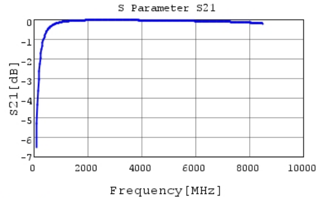
GRM0332C2A8R5WA01 S21 DCOV, 20degC
