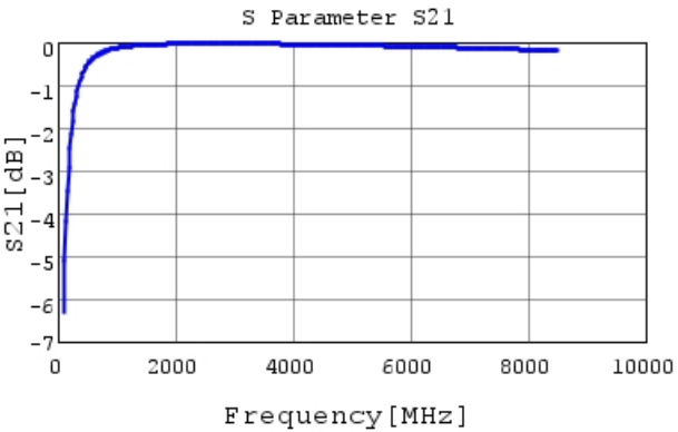
GRM0332C2A8R8CA01 S21 DCOV, 20degC
