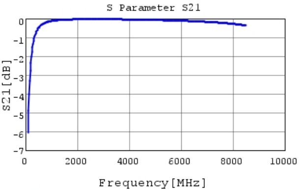
GRM0332C2A9R1DA01 S21 DCOV, 20degC
