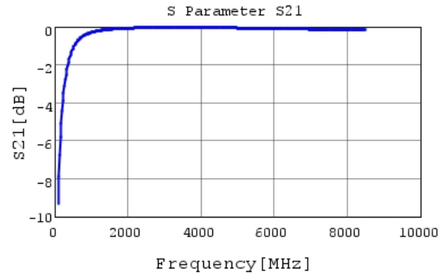
GRM0335C1H5R8BA01 S21 DCOV, 25degC
