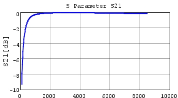
GRM0335C1H5R8CA01 S21 DCOV, 25degC
