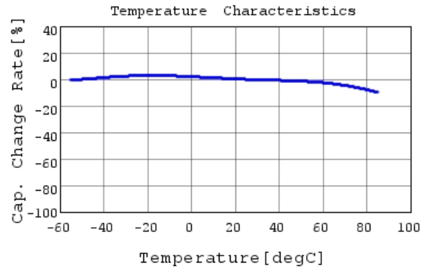
GRM033R60G224ME15 C-Temp. capchange, DC0.0V,
