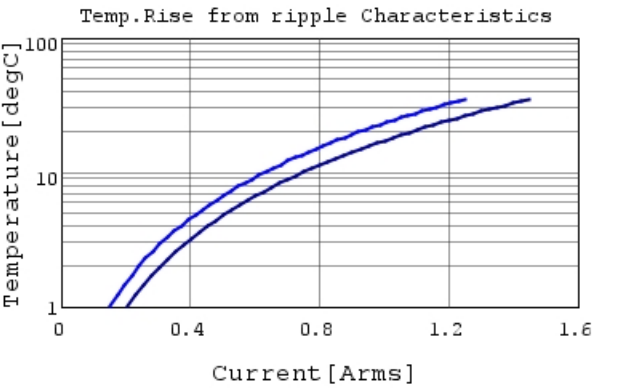
GRM033R60G224ME15 Temp.rise 600kHz
