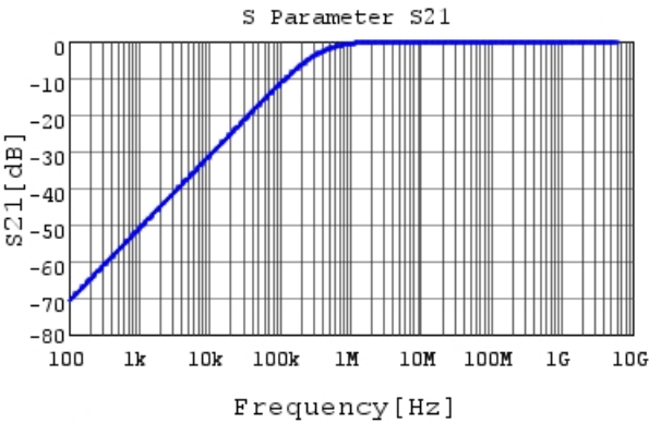
GRM033R61E472KA12 S21 DC0V,25degC
