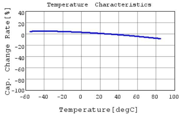
GRM033R61E472KA12 C-Temp. capchange, DC0.0V,
