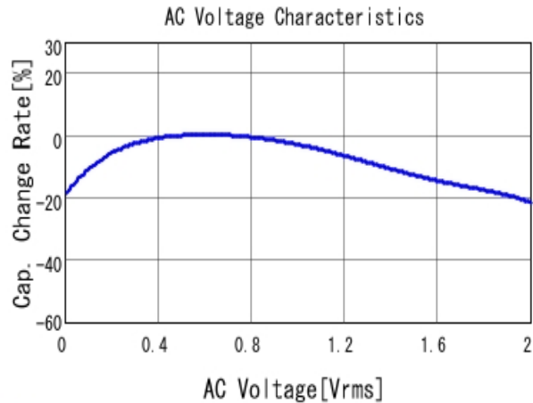
■ GRM035R60J475ME15 C-AC Voltage capchange, DCOV, 25.0d
