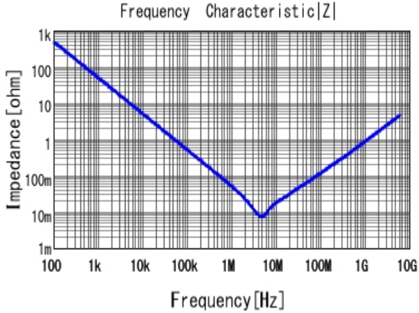
■ GRM035R60J475ME15 |Z| DCOV, 25degC
