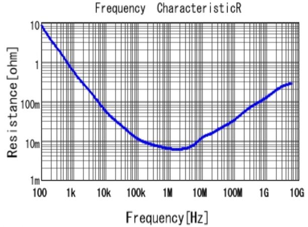
■ GRM035R60J475ME15 R DCOV, 25degC
