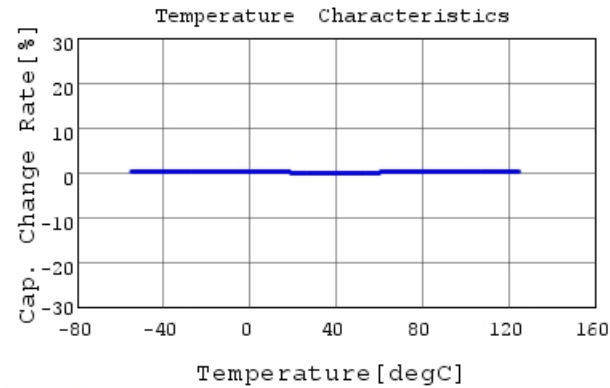
GRM1552C1H7R5BA01 C-Temp. capchange, DC0V, 1
