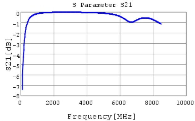
GRM1552C1H7R5BA01 S21 DC0V, 20degC
