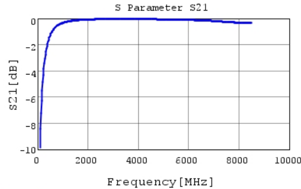
GRM1552C2A5R4DA01 S21 DC0V, 20degC
