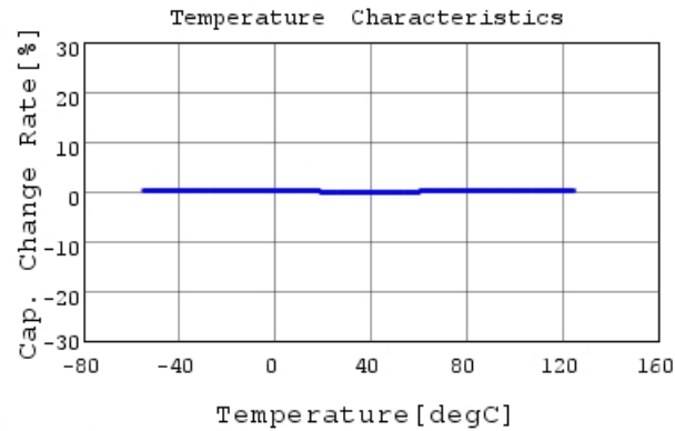
GRM1552C2A5R4DA01 C-Temp. capchange, DC0V, 1
