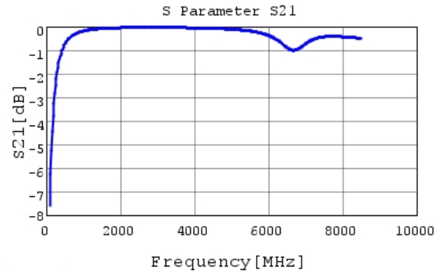
GRM1552C2A7R3WA01 S21 DCOV, 20degC
