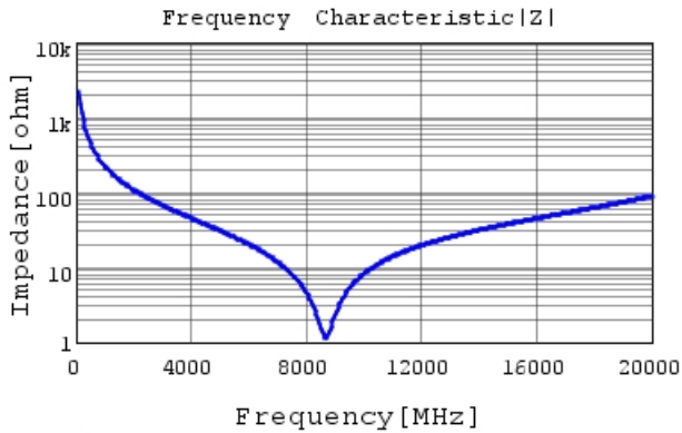
GRM1555C1HR70WA01 |Z| DCOV, 25degC
