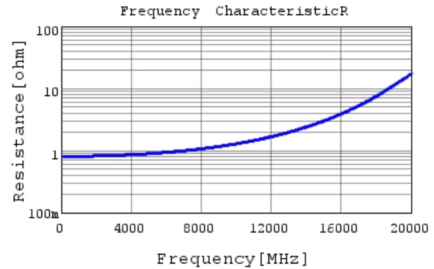
GRM1555C1HR70WA01 R DCOV, 25degC
