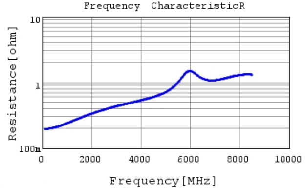
GRM1555C2A8R4CA01 R DCOV, 25degC
