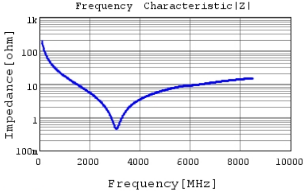
GRM1555C2A8R4CA01 |Z| DCOV, 25degC
