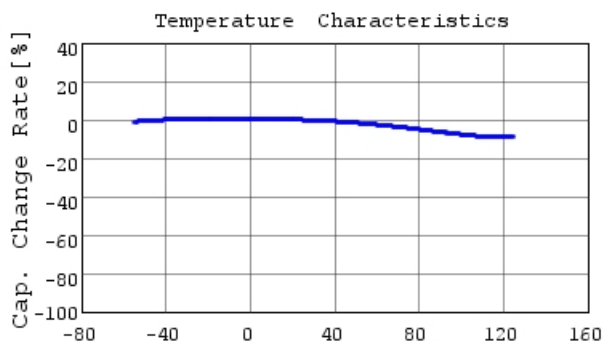
GRM155R71E473JA88 C-Temp. capchange, DC0.0V,
