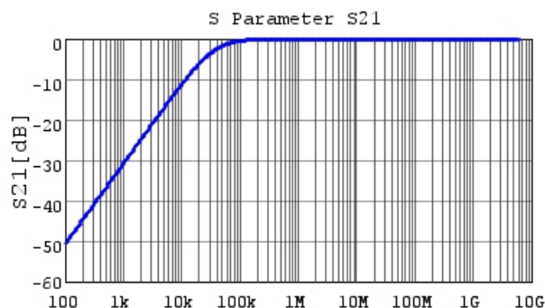
GRM155R71E473JA88 S21 DC0V,25degC
