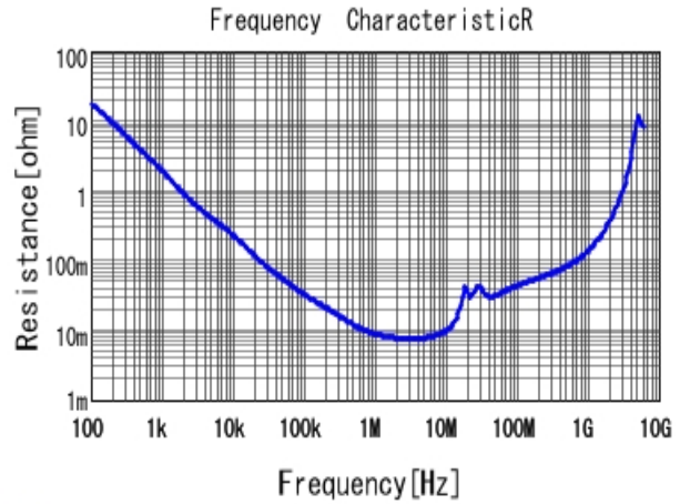
■ GRM21BR71H474KA88 R DCOV, 25degC
