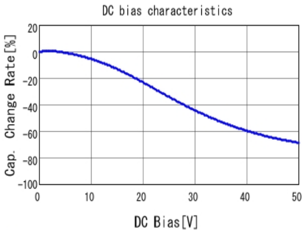
■ GRM21BR71H474KA88 C-DC bias capchange, 25.0degC, AC1.
