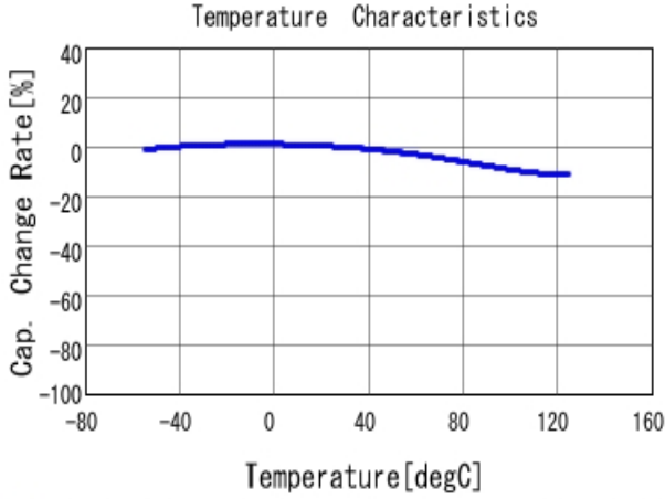
■ GRM21BR71H474KA88 C-Temp. capchange, DC0.0V, AC1.0V r m
