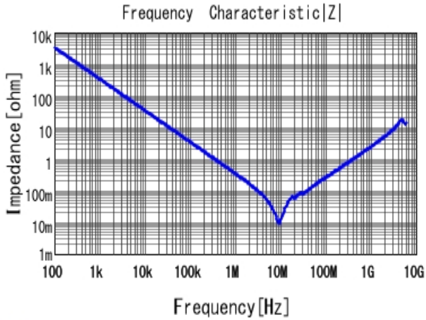
■ GRM21BR71H474KA88 |Z| DCOV, 25degC
