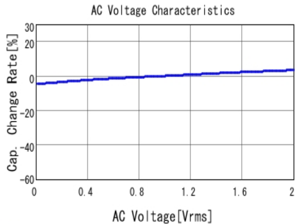
■ GRM21BR71H474KA88 C-AC Voltage capchange, DCOV, 25.0d
