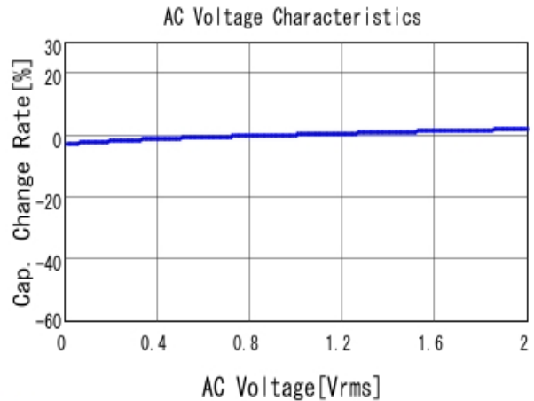
■ GRM21BR72A473KA01 C-AC Voltage capchange, DCOV, 25.0d
