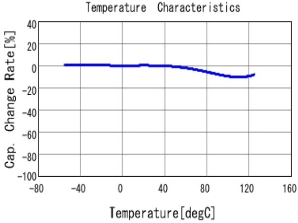
■ GRM21BR72A473KA01 C-Temp. capchange, DCO. 0V, AC1.0Vrm
