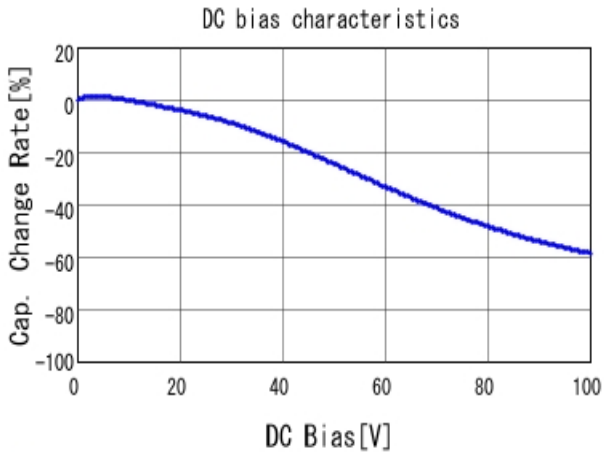
■ GRM21BR72A473KA01 C-DC bias capchange, 25.0degC, AC1.
