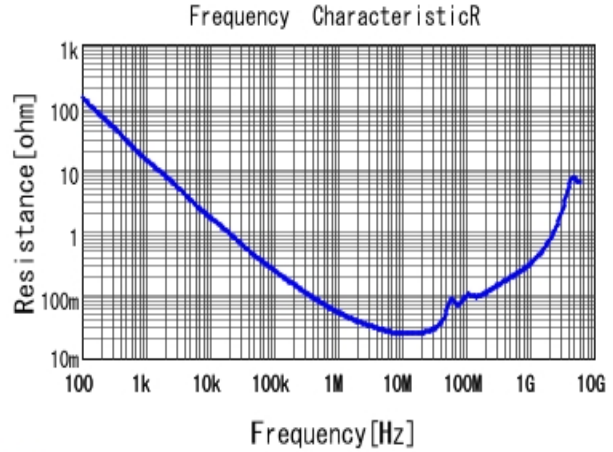
■ GRM21BR72A473KA01 R DCOV, 25degC
