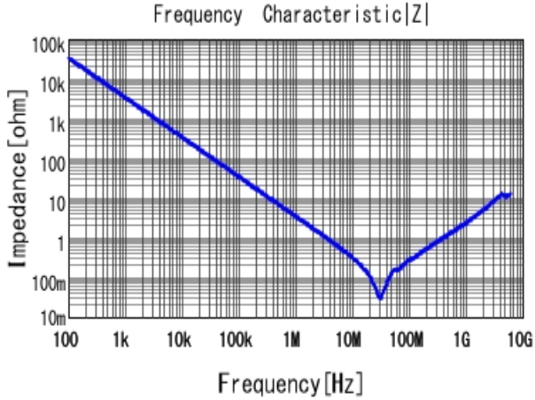
■ GRM21BR72A473KA01 |Z| DCOV, 25degC
