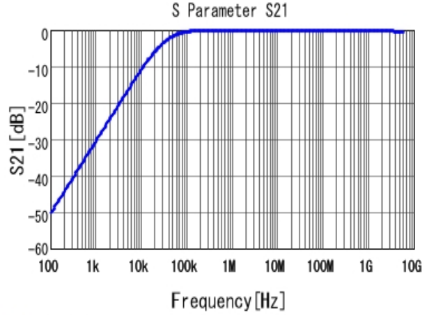
■ GRM21BR72A473KA01 S21 DCOV, 25degC
