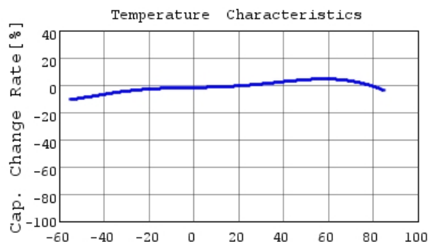
GRM31CR60J226KE19 C-Temp. capchange, DC0.0V,
