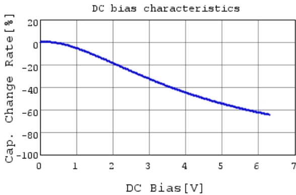
GRM32ER60J107ME20 C-DC bias capchange, 25.0
