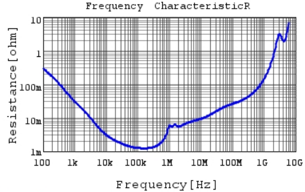
GRM32ER60J107ME20 R DCOV,25degC
