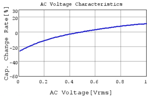
GRM32ER60J107ME20 C-AC Voltage capchange, D
