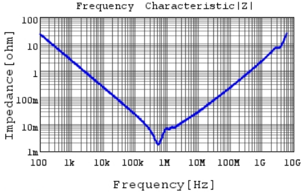
GRM32ER60J107ME20 |Z| DCOV,25degC
