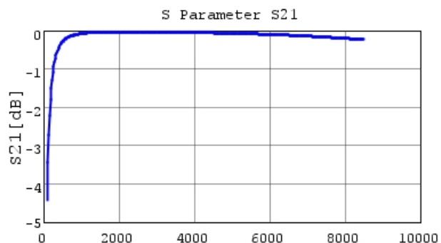
Frequency [MHz] GRT0335C1H120JA02 S21 DCOV, 25degC
