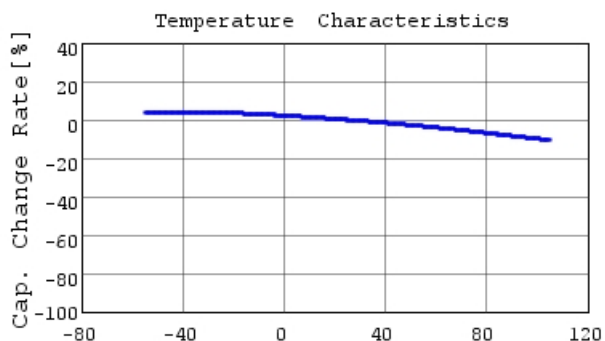
■ GRT033C80J682KE01 C-Temp. capchange, DC0.0V,
