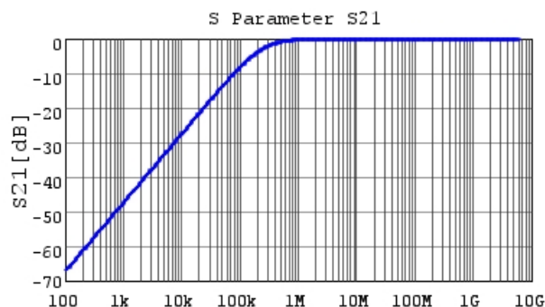
■ GRT033C80J682KE01 S21 DC0V, 25degC
