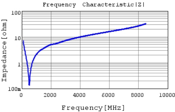
GRT1555C1E221JA02 |Z| DCOV,25degC
