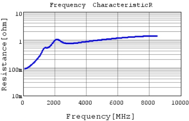
GRT1555C1E221JA02 R DCOV,25degC
