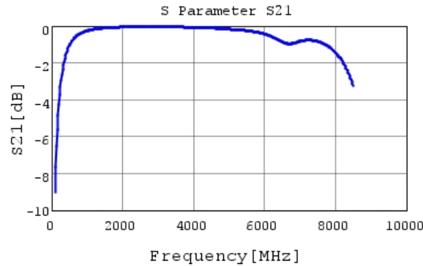
GRT1885C1H6R0DA02 S21 DCOV, 25degC
