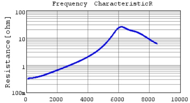
GRT1885C2A100JA02 R DCOV,25degC
