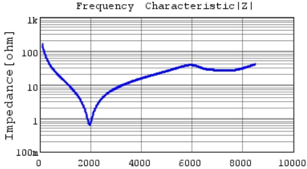
GRT1885C2A100JA02 |Z| DCOV,25degC
