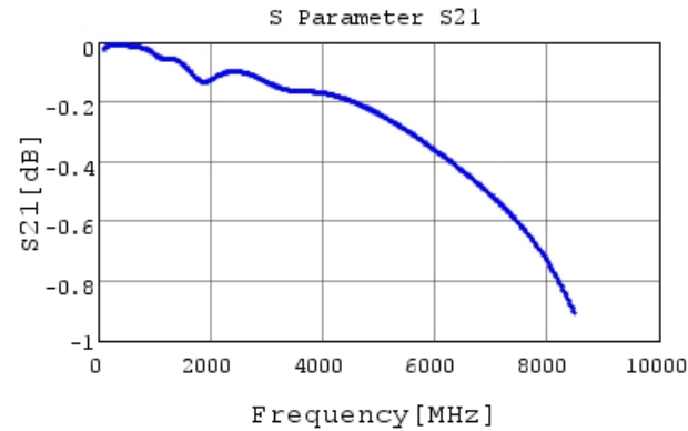
GRT1885C2A221JA02 S21 DCOV, 25degC
