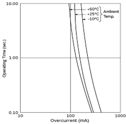
Operating Time (Typical Curve)
