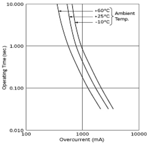
Operating Time (Typical Curve)
