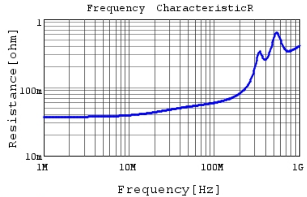
RDE5C2A222J1K1H03B R DCOV, 25degC
