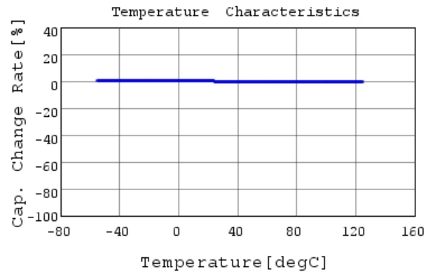
RDE5C2A222J1K1H03B C-Temp. capchange, DCOV,
