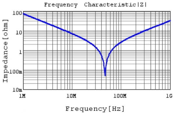
RDE5C2A222J1K1H03B |Z| DCOV, 25degC
