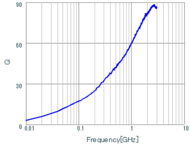
LQG15WH2N3C02 Q.
