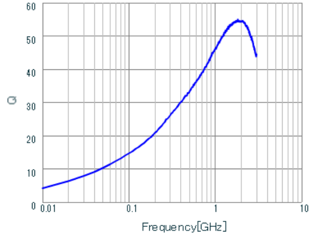
LQG15WZ7N3G02 Q.
