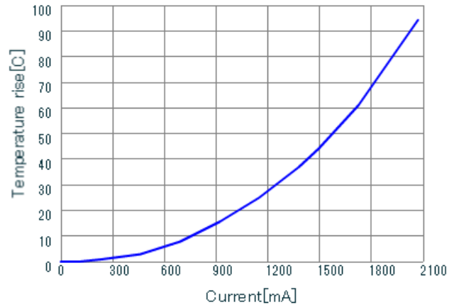
LQH3NPN6R8MMR DT_Current
