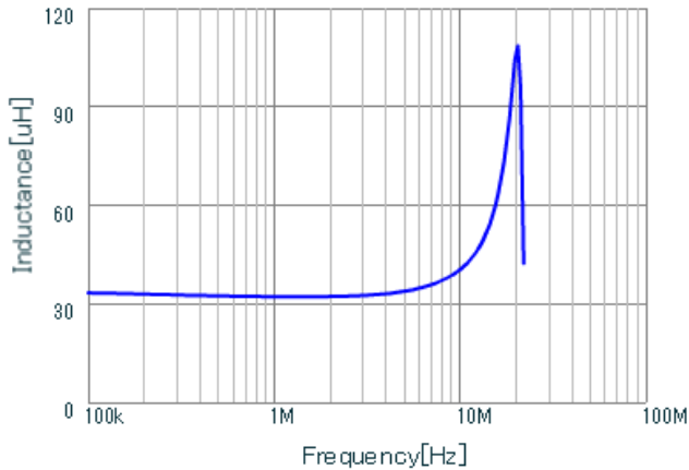
LQH44PZ330MGR L
