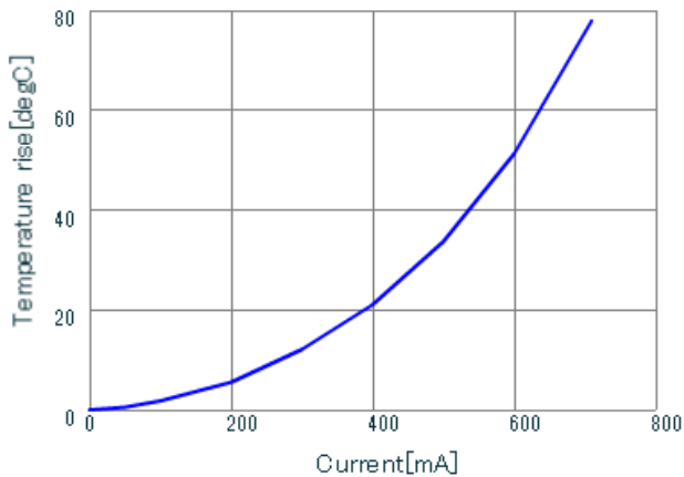
LQH44PZ330MGR DT_Current
