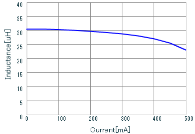
LQH44PZ330MGR DC-Bias, 20
