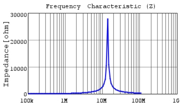
LQH5BPN220M38 |Z|
