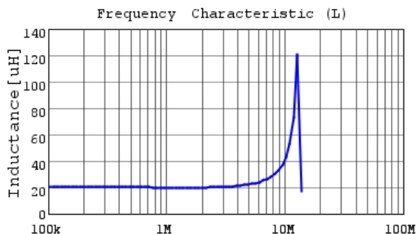
LQH5BPN220M38 L
