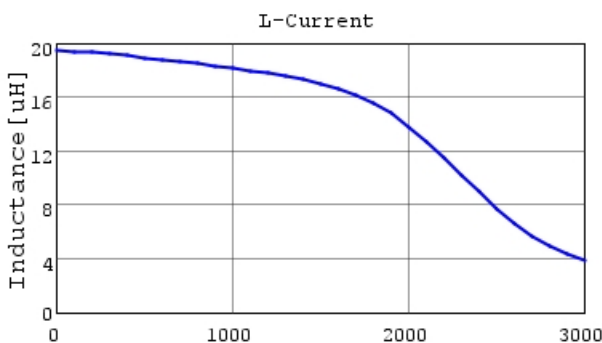
LQH5BPN220M38 L-Current 20degC
