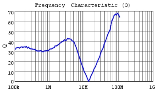
LQH5BPN220M38 Q
