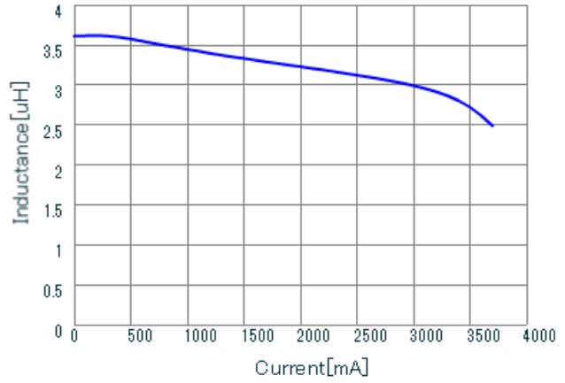
LQH5BPN3R3NT0 DC-Bias, 20
