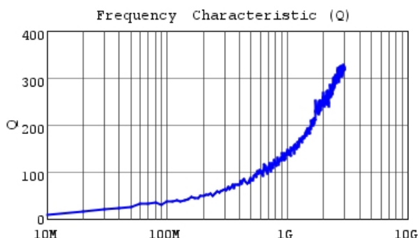
LQP03TN0N7CZ2 Q
