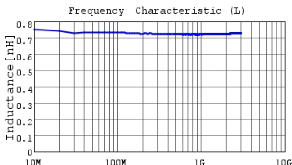
LQP03TN0N7CZ2 L
