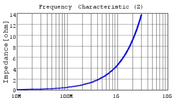
LQP03TN0N7CZ2 |Z|
