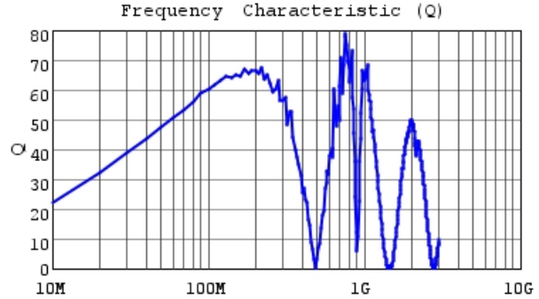
LQW2UASR62G0C Q
