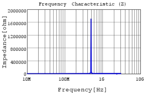
LQW2UASR62G0C |Z|
