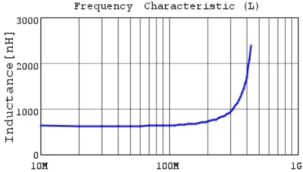
LQW2UASR62G0C L
