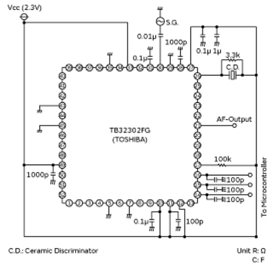
Measurement Circuit
