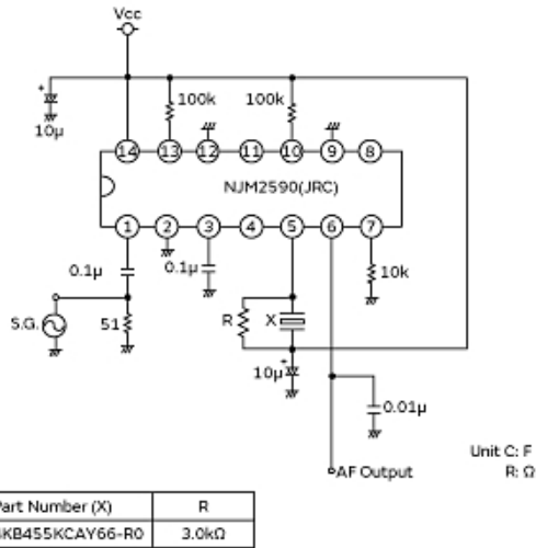
Measurement Circuit
