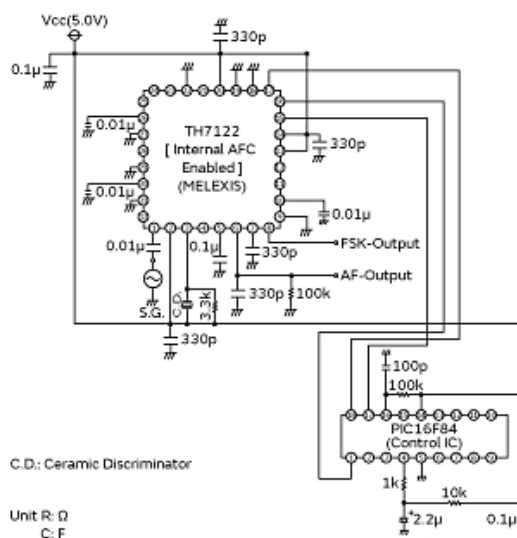
Measurement Circuit
