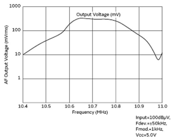
Frequency Characteristics
